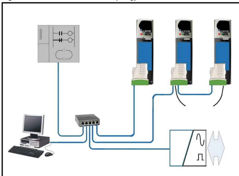
Figure 4-3 SM-PROFINET network topology
